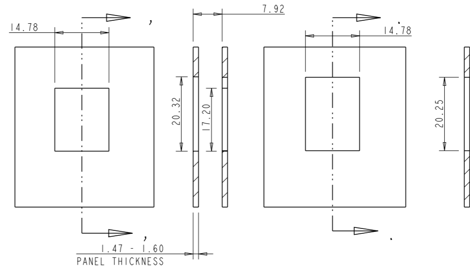
SUGGESTED FLUSH MOUNT PANEL APPLICATION CUTOUT SINGLE PANEL CUTOUT
